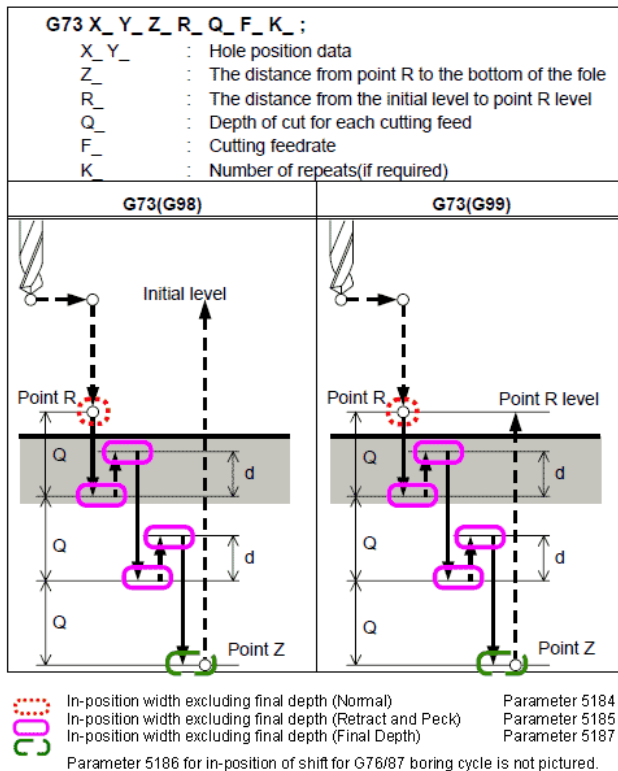
High-Speed peck Drilling Cycle (G73)
